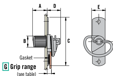
Nylon knob
