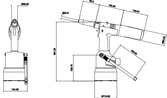
Quick release stem collector bottle option (71213 series)
