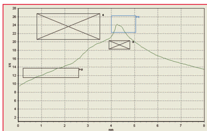
A) Correctly installed fastener: curve is correct
