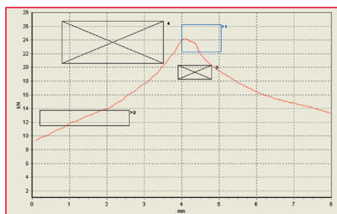
B) Incorrectly installed fastener: curve is incorrect
